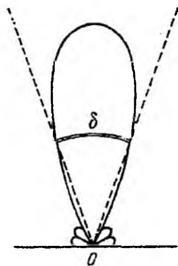
63-rasm. Radioteleskopning yo‘nalganlik diagrammasi
