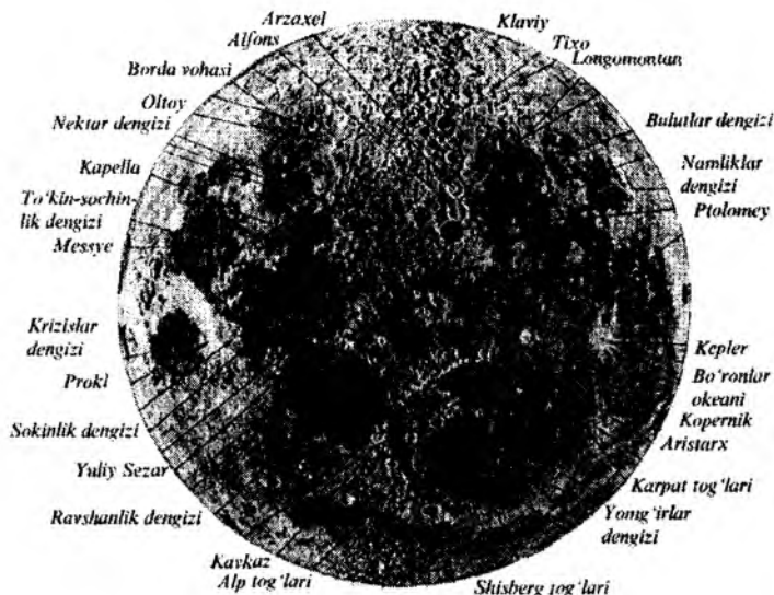
97-rasm. Oy relyefining tasvirlanishi
