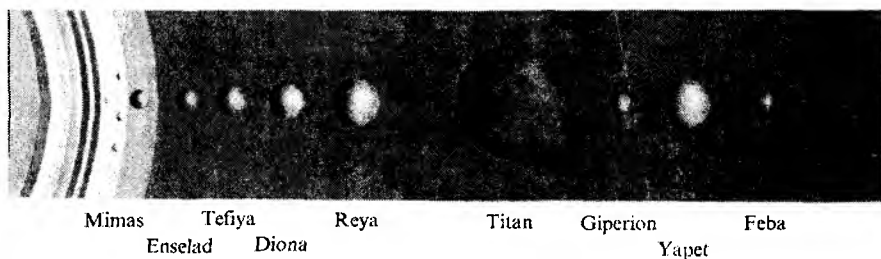
109-rasm. Saturnning yirik yo‘ldoshlari
