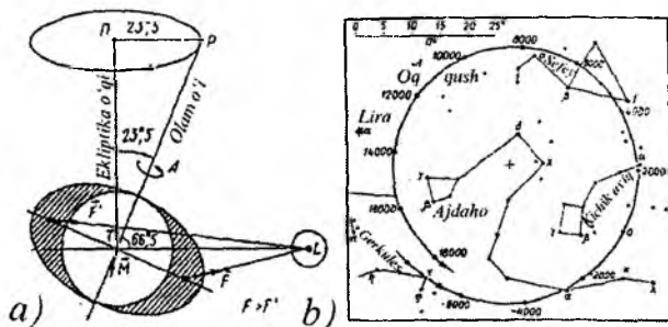
41-rasm. Pretsessiya hodisasini tushuntirish
