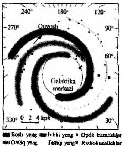
148-rasm. Galaktikamizning yenglari va unda Quyoshning o'rni
