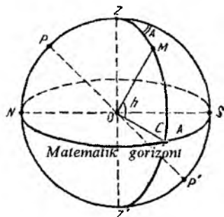
4-rasm. Gorizontalar sistemasi
