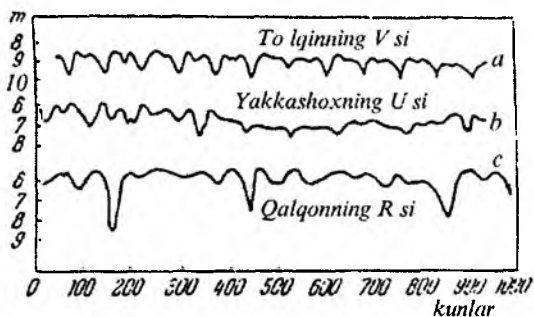
142-rasm. Savrning RV tipidagi yulduzlar ravshanligining o'zgarishi
