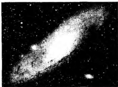
149-rasm. Galaktikamizga qo'shni Andromeda galaktikasi
