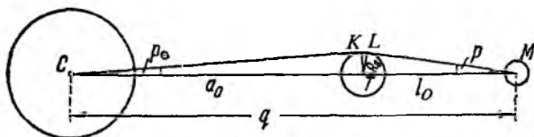
36-rasm. Quyoshning sutkalik gorizontaI paralaksini aniqlash usuli
