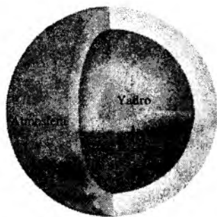
113-rasm. Neptun va uning ichki tuzilishi
