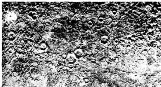
92-rasm. Merkyriyning «Mariner-10» olgan relyefi
