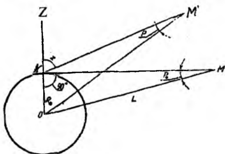
19-rasm. Yoritgichlarning sutkalik va sutkalik-gorizontal parallaksleri
