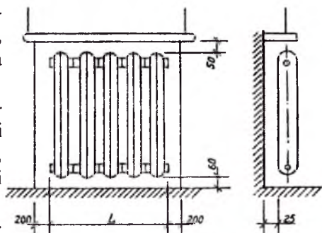
4.17-rasm. Radiatorlarning mehroblarga o'rnatilishi
