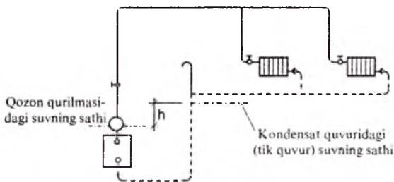
9.1-rasm. Past bosimli bug'li isitish tizimining soddalashtirilgan sxemasi
