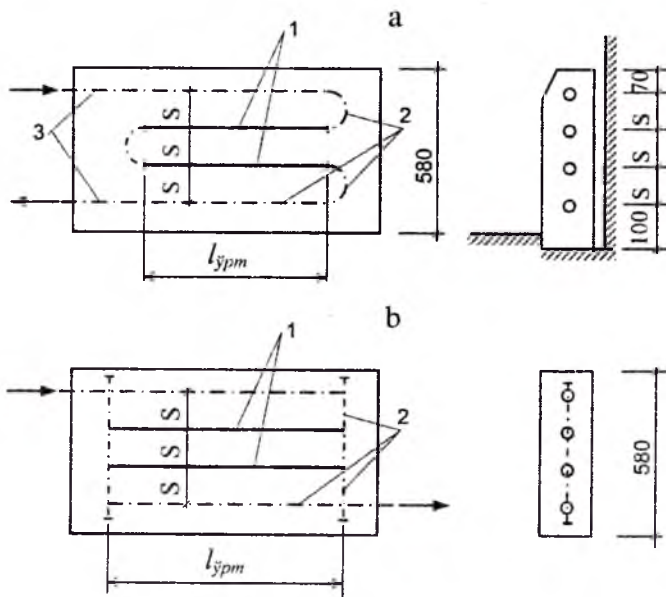
11.2-rasm. Egilib va ustunchali qilib yasalgan isitish panellarning sxemasi
