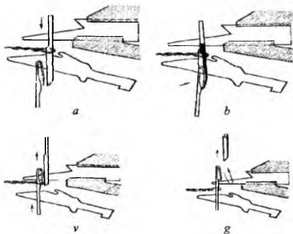
4.17-rasm. Koton mashinasida halqa ko'chirish jarayoni.
