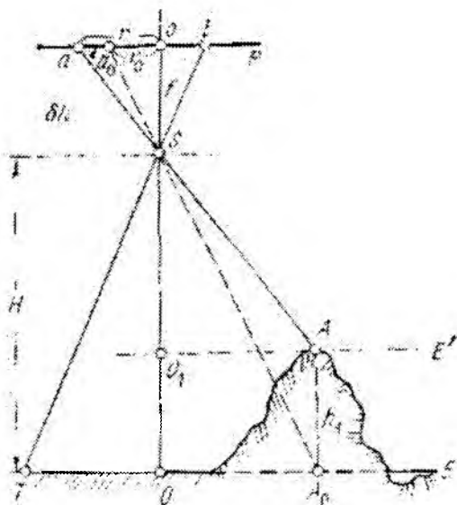
4.15-rasm. Joy reliefi ta'sirida aerofotosuratda nuqtaning siljishi
