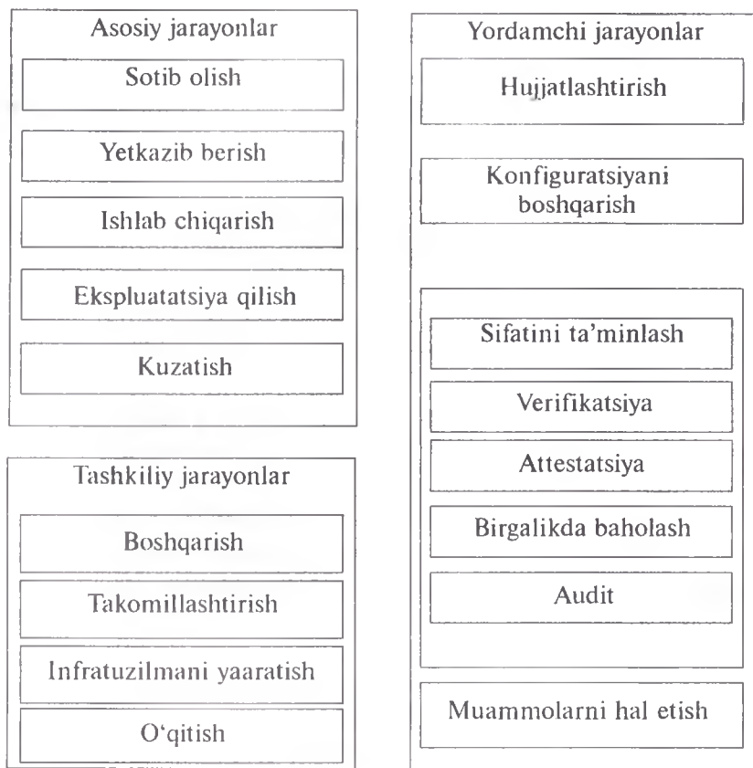
1.9-rasm. Dasturiy ta'minot hayotiy zanjiri jarayonining tuzilmasi.
