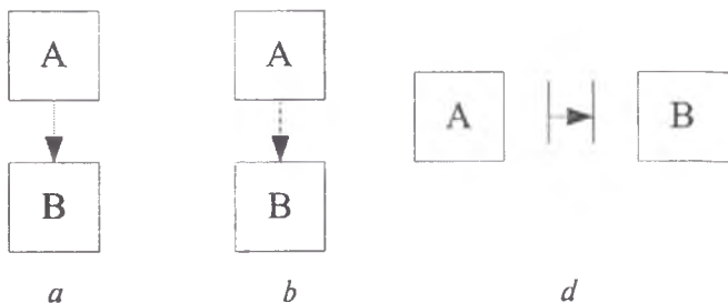
5.8-rasm. Chaqiruv tiplari belgilanishi: a – bosqichli chaqiruv; b – parallel chaqiruv; d – hamdastur chaqiruv.
