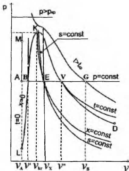
1.6-rasm. Suv bug'ining fazaviy ( p, v ) - diagrammasi
