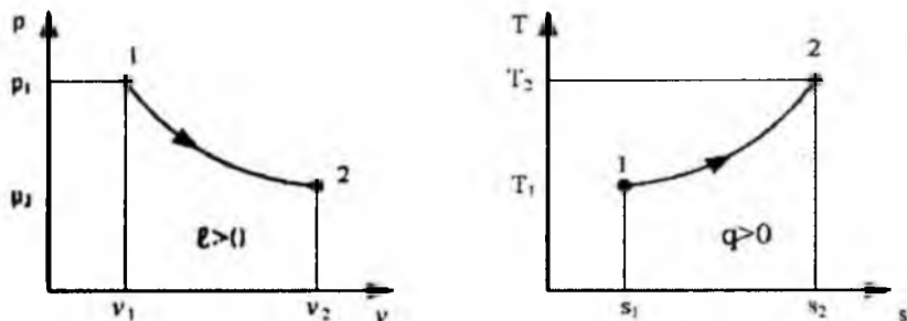
1.4-rasm. Ideal gazning p, v - va T, s - diagrammalardagi politrop kengayish jarayoni ( n=0,4 ).
