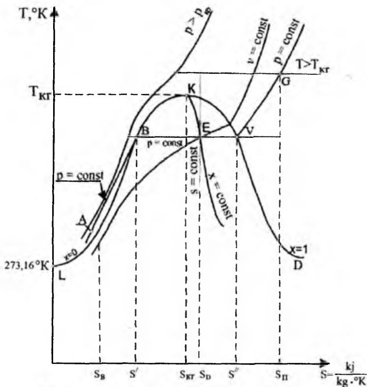
1.7-rasm. Suv bug'ining fazaviy (T, s) – diagrammasi
