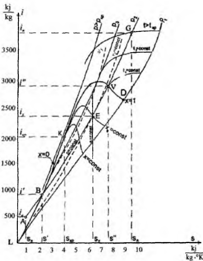
1.8-rasm. Suv bug'ining fazaviy (i, s) – diagrammasi
