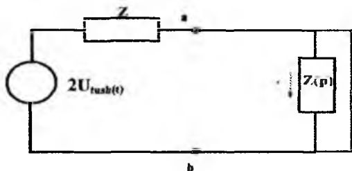
7.6- rasm. Liniyada singan to'liqning amplimtudasini aniqlash uchun foydalaniluvchi almashtirish sxemasi: Z(p) – tugunning ekvivalent qarshiligining operator ko'rinishida ifodalanishi.
