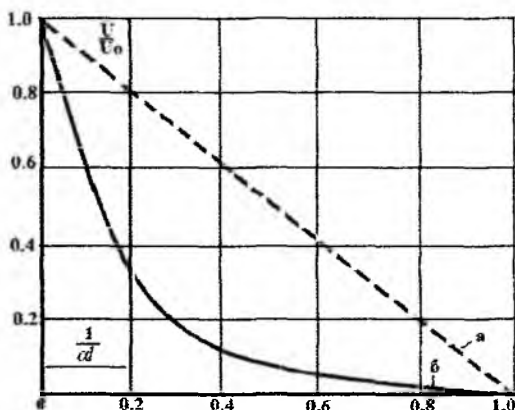
5.6- rasm. cd = 5 ga teng bo'lgan chulg'am bo'ylab kuchlanishning bosqlang'ich taqsimlanishi. a – neytral izolyatsiyalangan; b – neytral zaminlangan.
