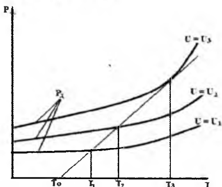
3.7- rasm. Issiqlikdan teshilish mexanizmgiga tushuntirish
