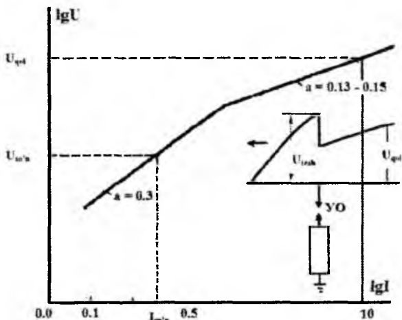
8.11- rasm. Ventilli razryadlagichning ishlash prinsipi va uning ishchi qarshiligini volt – amper xarakteristikasi (razryadlagich diskining diametri d = 130 mm, I kiloamperda)
