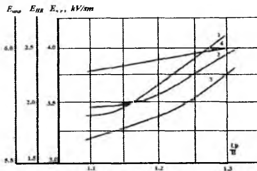
4.6- rasm. Likopsimon izolyator uchun o'rtacha razryadlanish kuchlanishining \frac{I_p}{H} nisbatga bog'liqligi: 1- o'rtacha quruq razryadlanish kuchlanishi ( E_{ov} ); 2- o'rtacha ho'l razryadlanish kuchlanishi gradiyenti ( E_{HR} ); 3- to'liq musbat qutbli impulslarda o'rtacha razryadlanish gradiyenti ( E ); 4- to'liq manfiy qutbli impulslarda o'rtacha razryadlanish kuchlanishi ( E_{imp} ).
