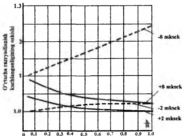
3.12- rasm. Tayanch izolyatorida qovurg'aning joylashish o'rining uning impuls razryadlanish kuchlanishiga ta'siri.
