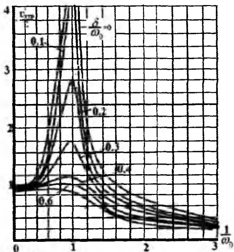
7.20- rasm. \frac{\delta}{\omega_0} ning har xil qiymatlari uchun rezonans egri chizig'i \frac{U_{c_{MAX}}}{E} = f\left(\frac{1}{\omega_0}\right) ning ko'rinishi
