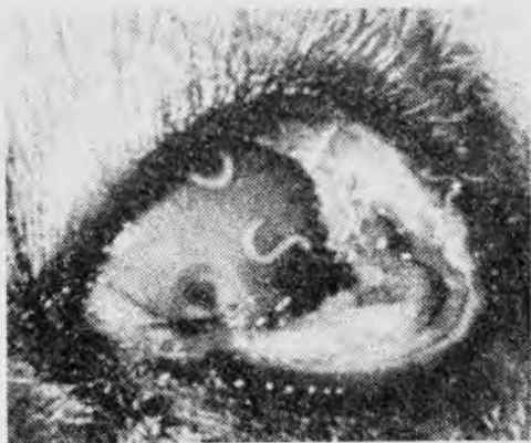
42-rasm. Qoramol ko'zidagi telyaziyalar
