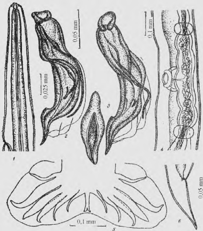
30-rasm. Trichostrongilyuslarning morfologiyasi: Trichostrongilus retortiformis (Zeder, 1800) Looss, 1905 (Shuls, 1931 buyincha) 1) tananing bosh qismi; 2) spikulalar; 3) rulek; 4) urg'ochi nusxanning jinsiy teshik (vulva) qismi; 5) erkak nusxaning jinsiy bursasi; 6) urg'ochi nusxaning dum qismi
