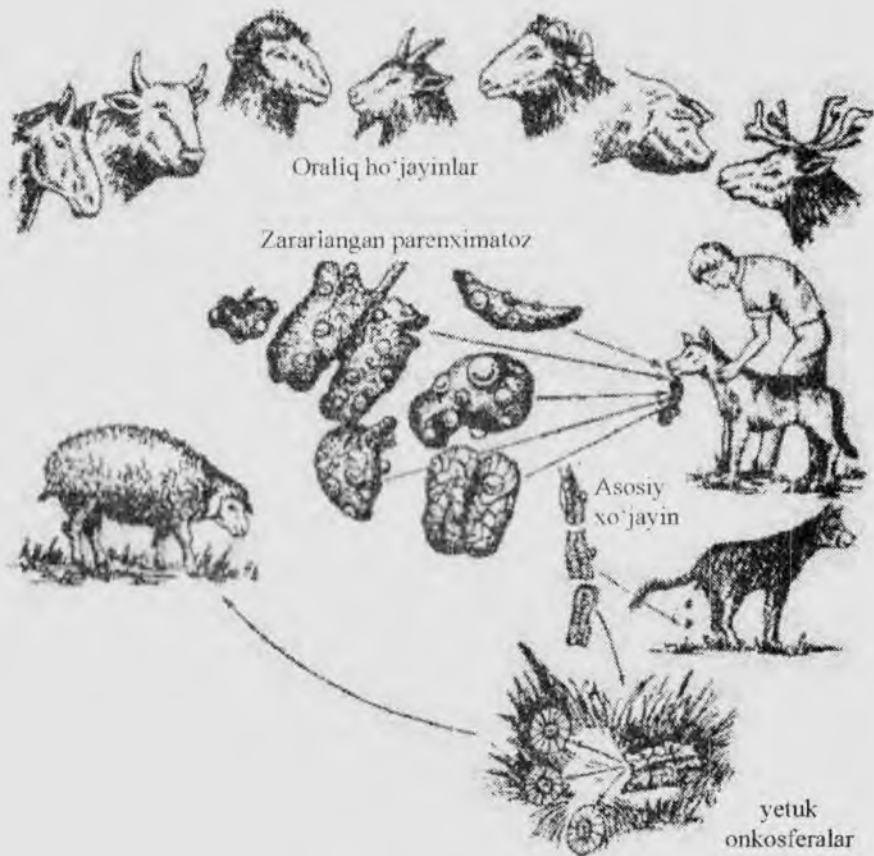
14-rasm. Exinokokklarning biologiyasi (Ergashev, Abduraxmonov, 1992)
