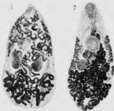
43-rasm. Prostogonimoz qo'zg'atuvchisi: 1- Prosthogonimus ovatus ; 2- Prosthogonimus cuneatus .
