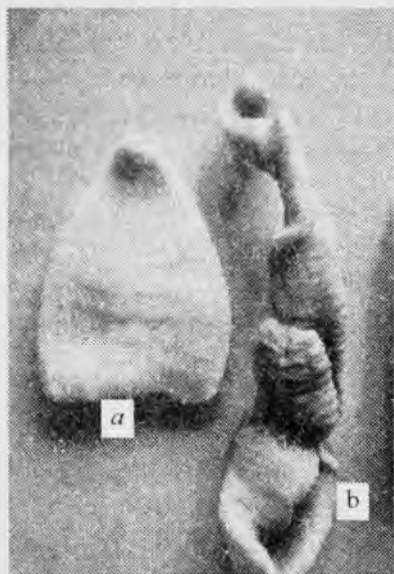
57-rasm. a - Anoplocephala magna ;
