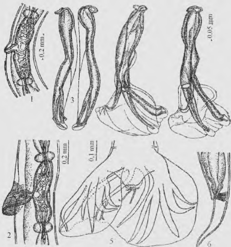
23-rasm. Marshallagiyalarning morfologiyasi: Marshallagia marshalli Ransom, 1907: 1. 2) urg'ochisining jinsiy organlari (Gushanskaya va Kryukova, 1930); 3, 4) spikulalar. 5) erkak nusxaning jinsiy bursasi (Gorshkov buyincha); 6) urg'ochi nusxaning dum qismi (Ransom, 1907 bo'yicha)
